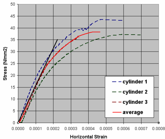
Figure 13. Stress versus horizontal strain
