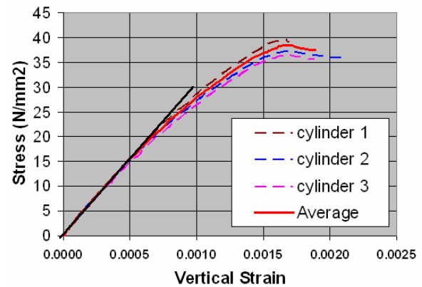
Figure 12. Stress versus vertical strain
